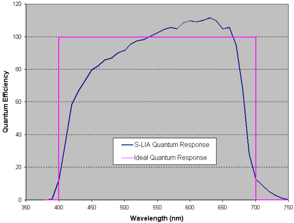
Figure 1: PAR Smart Sensor Typical Quantum Response
